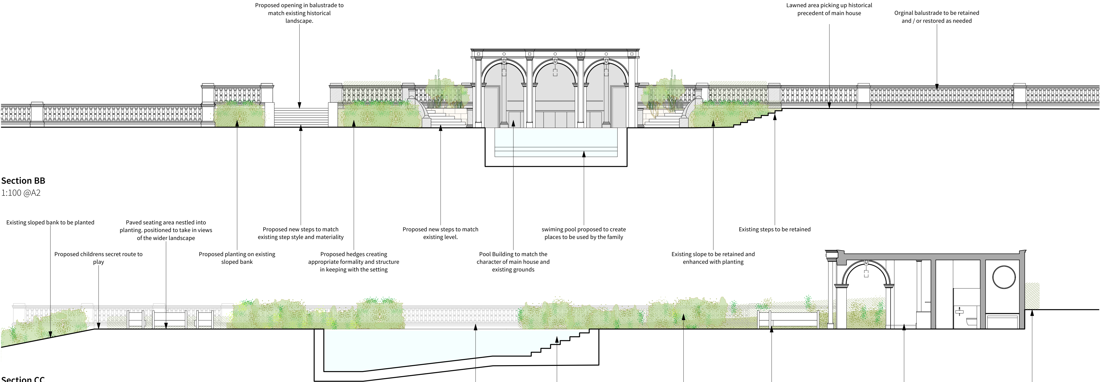
Section CC 1:100 @A2
