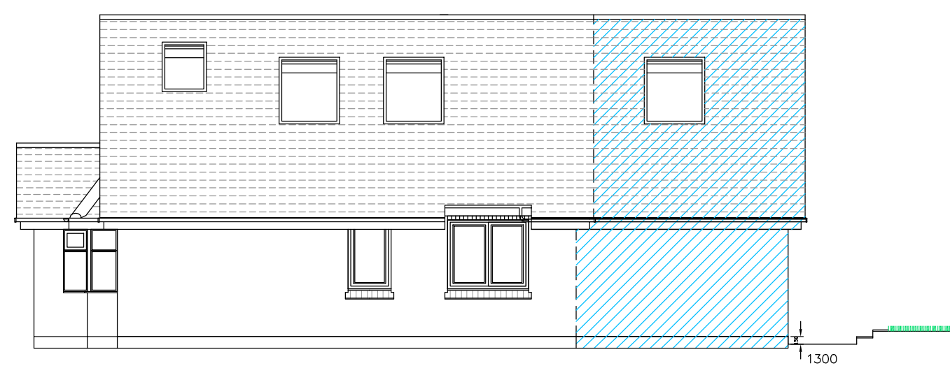
Proposed Side (North) Elevation
