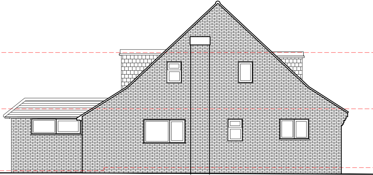
B) Existing Side Elevation
