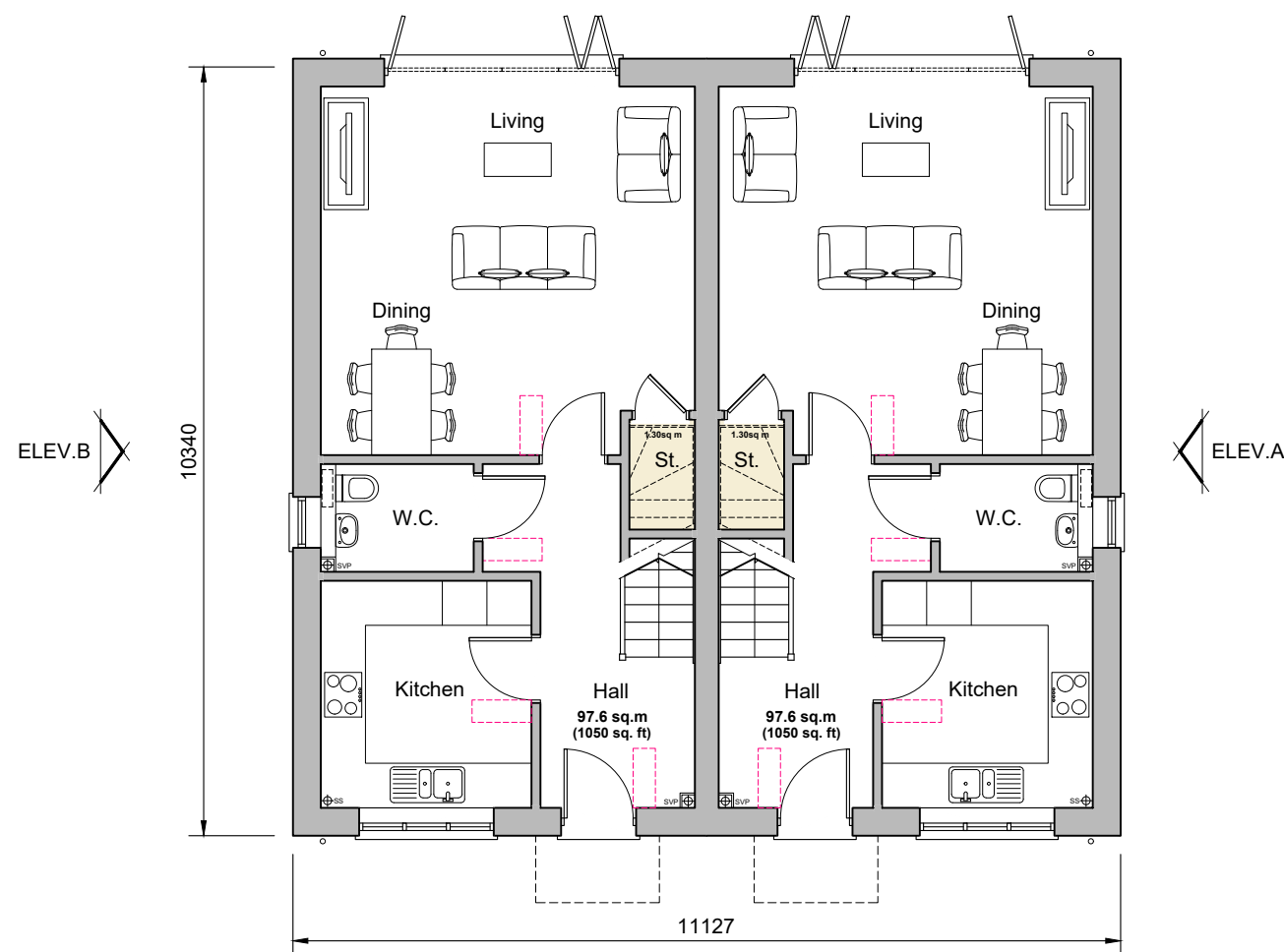
Ground Floor Plan Plots 11-12
