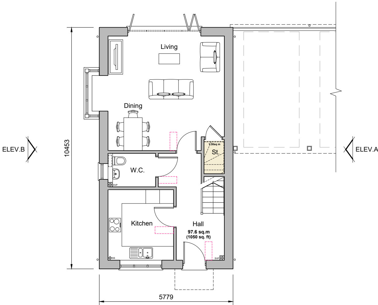
Ground Floor Plan Plot 13 Plot 14 (handed)
