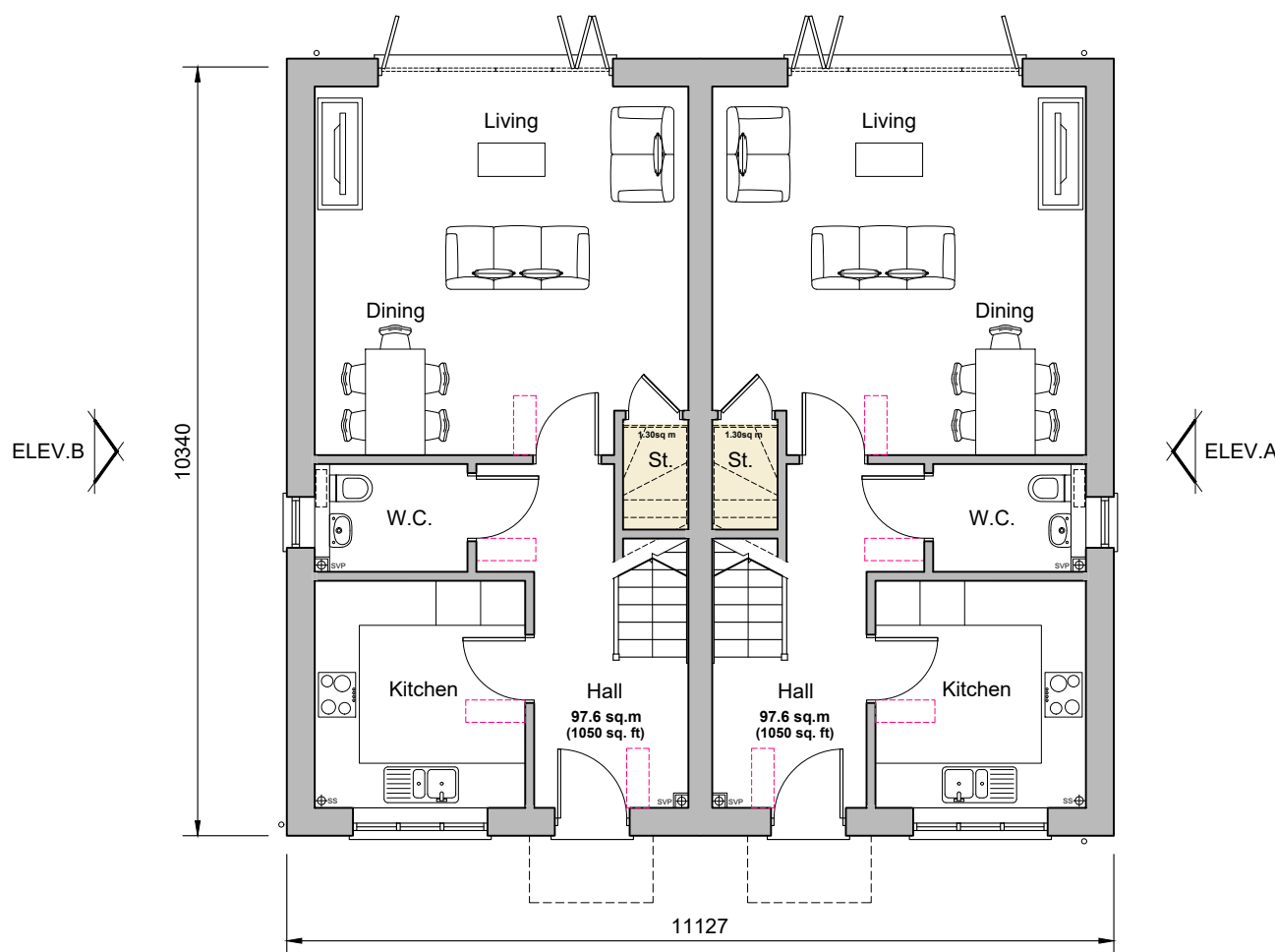
Ground Floor Plan Plots 18-19
