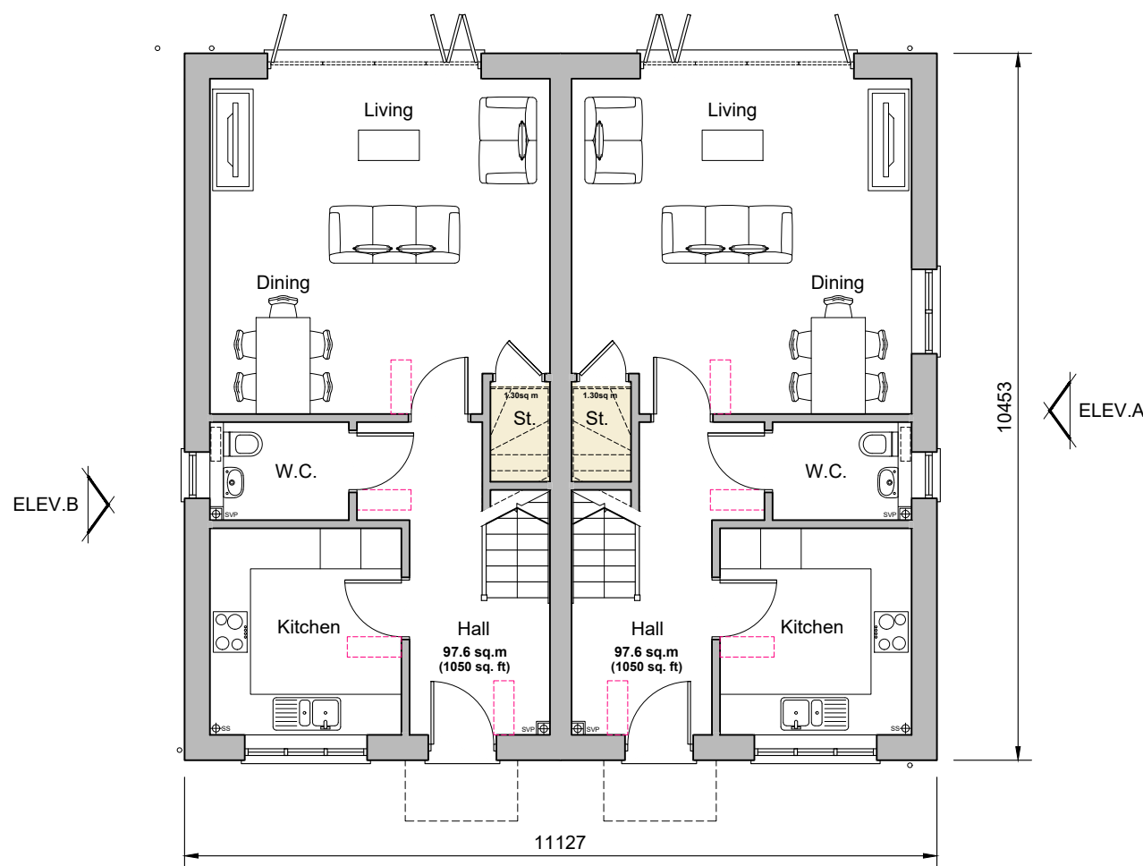
Ground Floor Plan Plots 6-7
