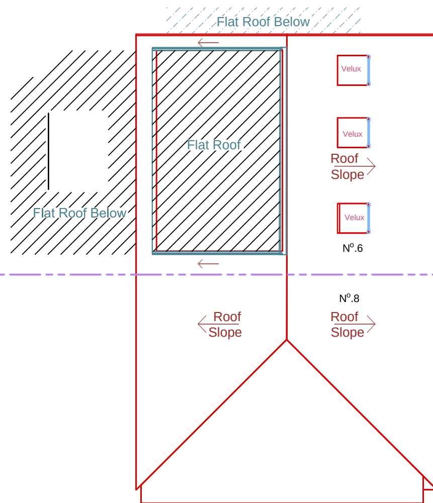
ROOF PLAN PROPOSED SCALE 1:100
