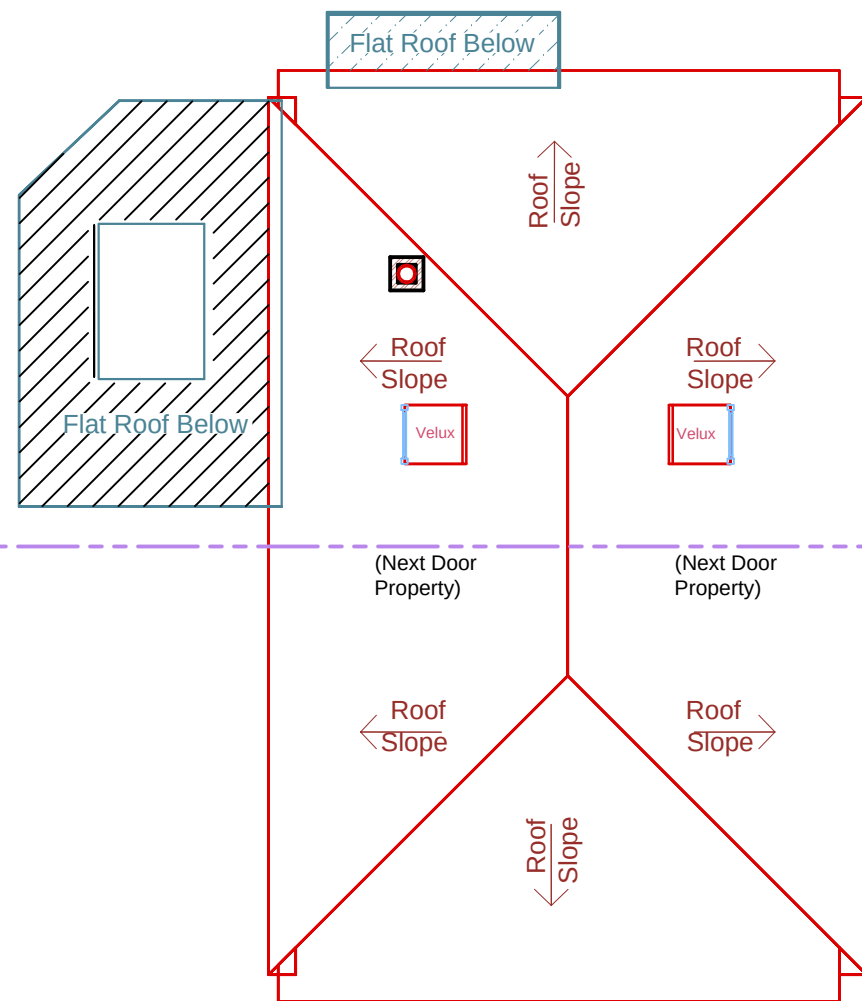
ROOF PLAN EXISTING SCALE 1:100
