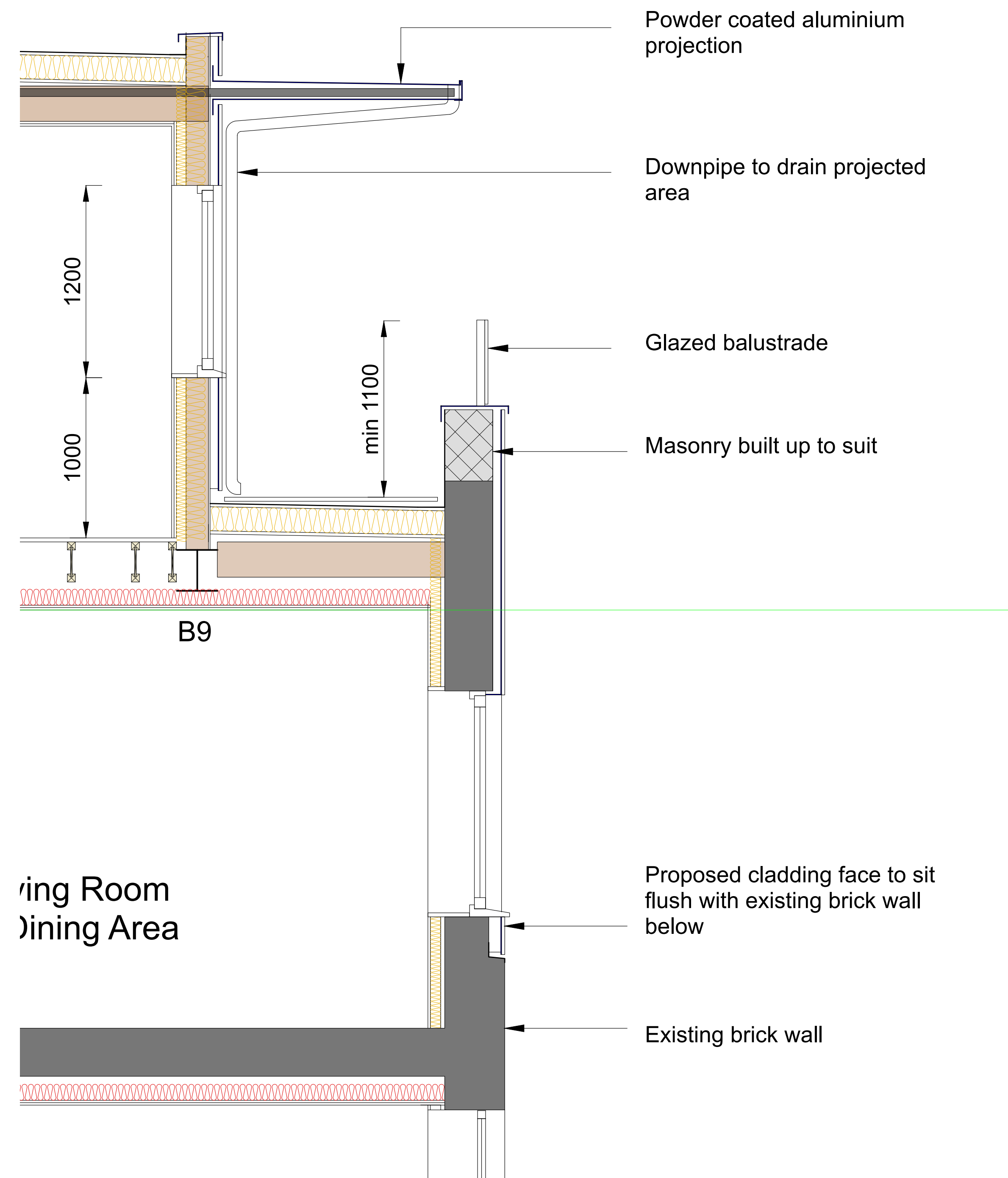
c) Perimeter upstand detail
