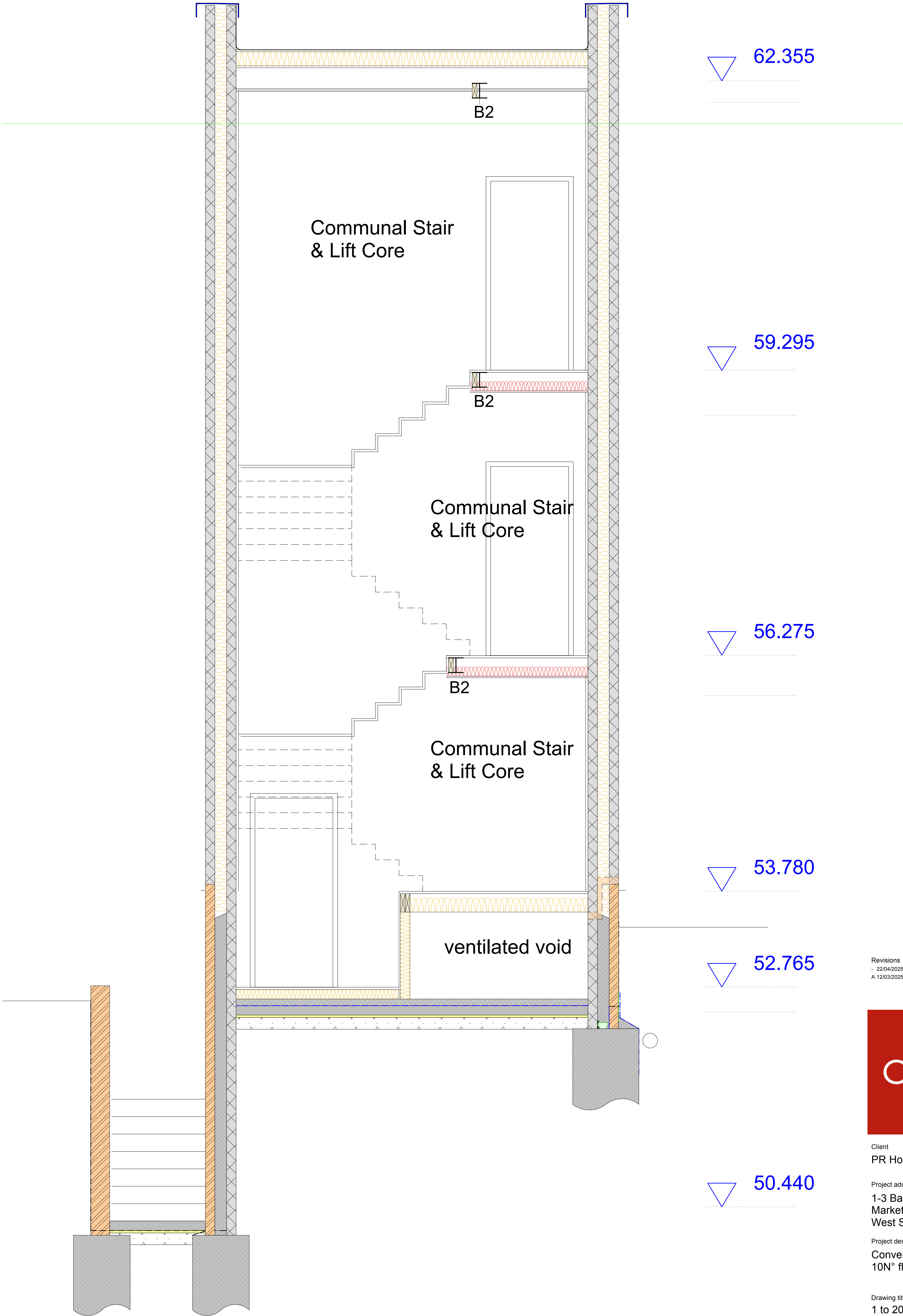
1 to 20 Section Stair and lift core for flats 3, 6 & 9
