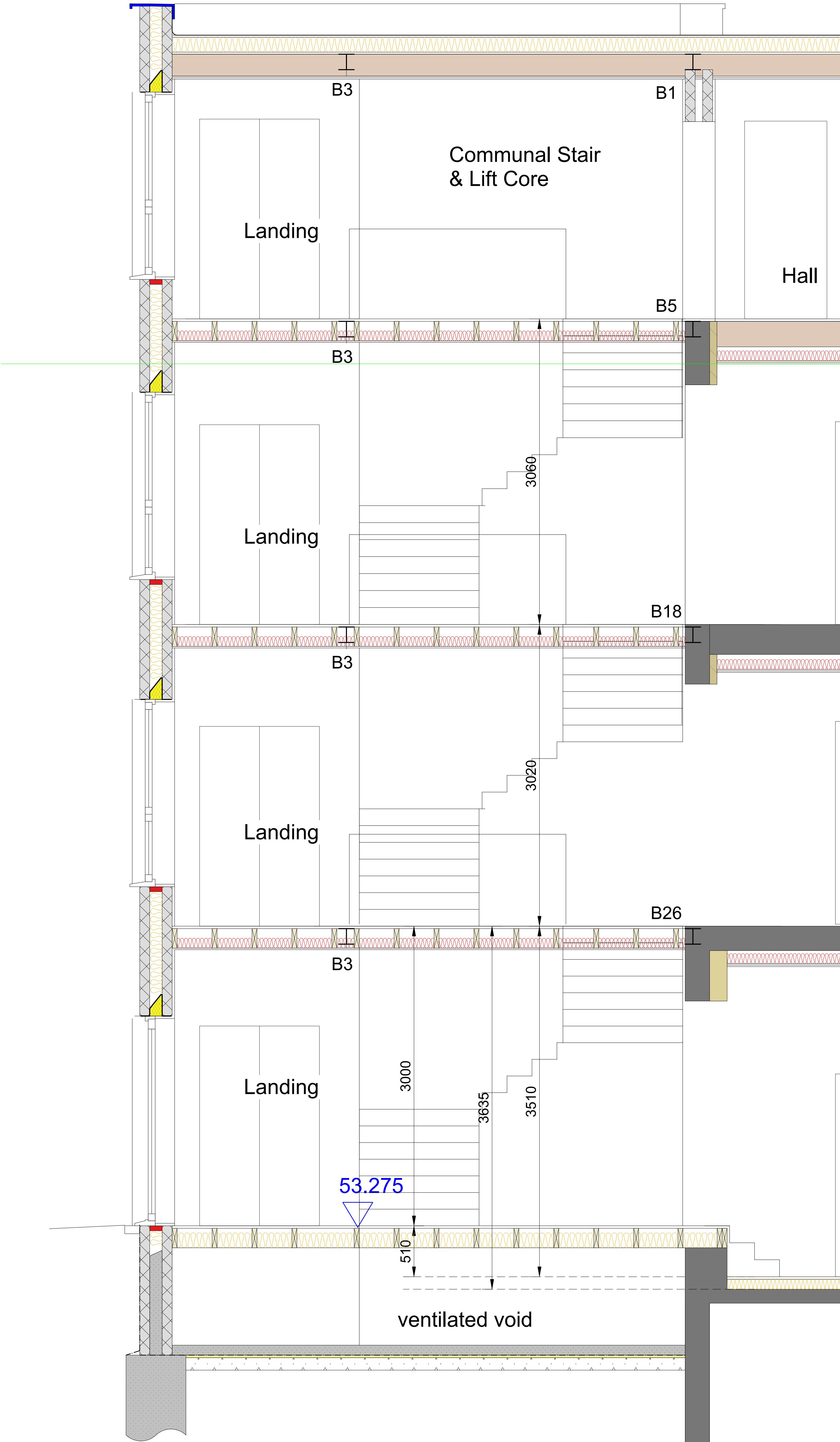
1 to 20 Section Stair and lift core for flats 1, 2, 4, 5, 7, 8 & 10
