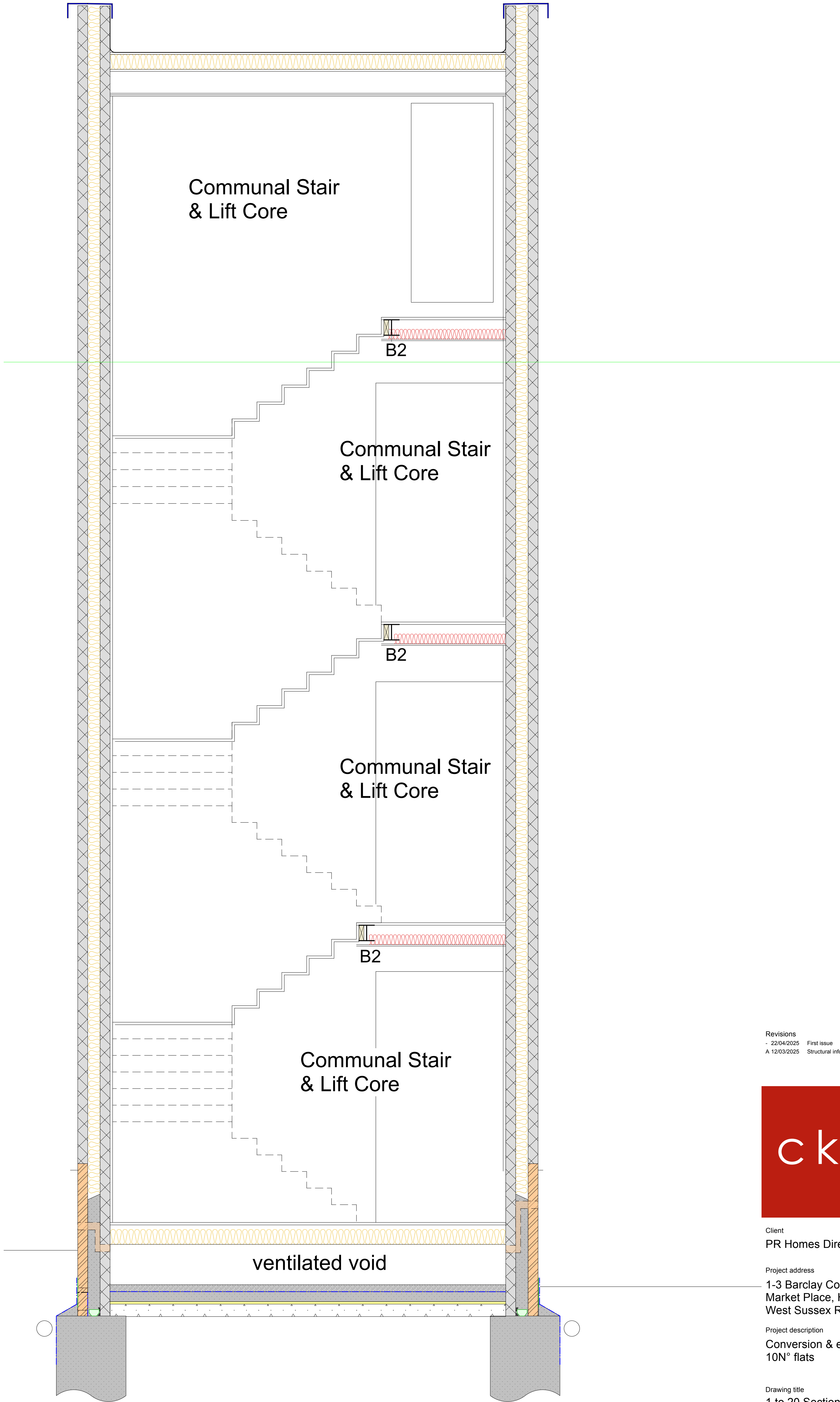
1 to 20 Section Stair and lift core for flats 1, 2, 4, 5, 7, 8 & 10
