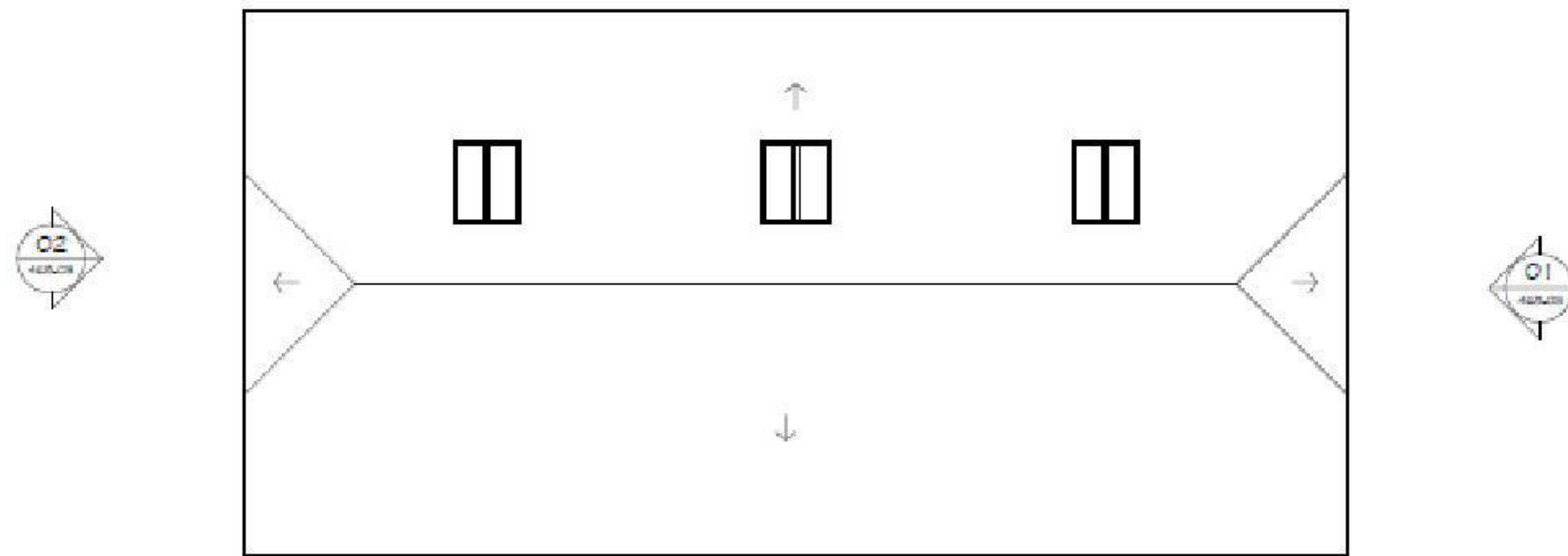
01 Roof Plan Scale 1:50 @ A1
