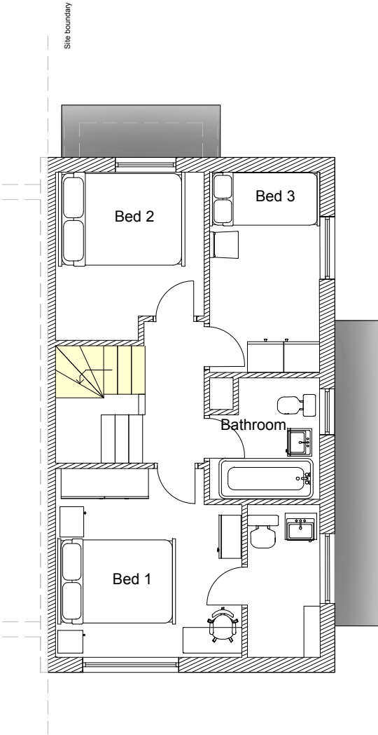
02 First floor plan - As Proposed 3000 1:100 (at A3)
