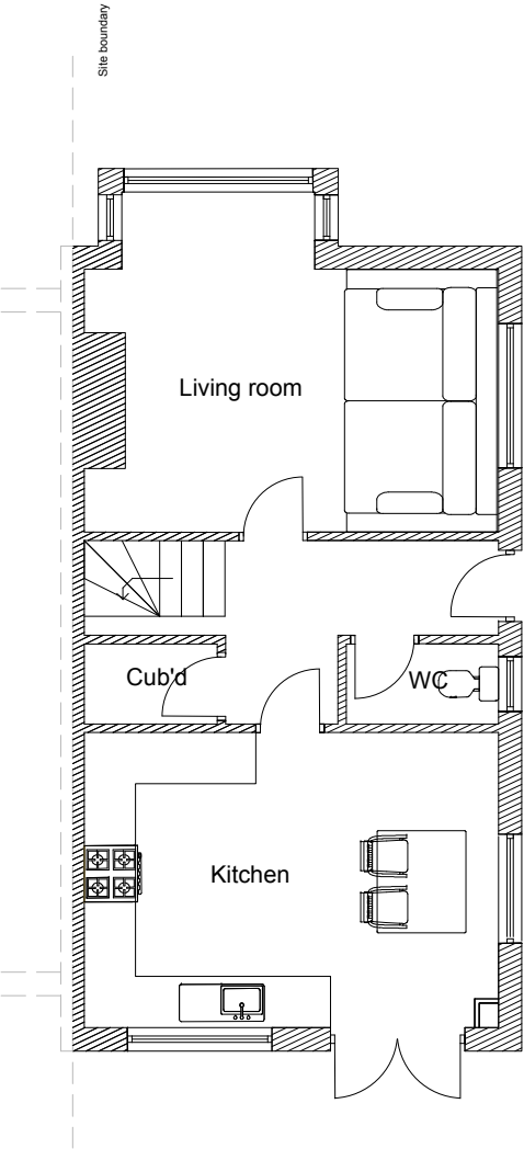
01 Ground floor plan - As Proposed 3000 1:100 (at A3)
