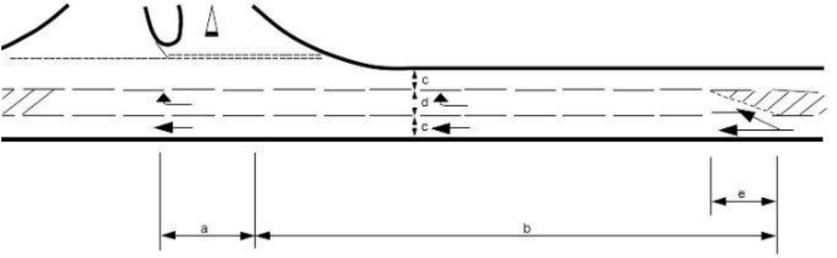
Figure 6.3b Major / minor priority junction with a up-gradient ghost island on climbing lane
